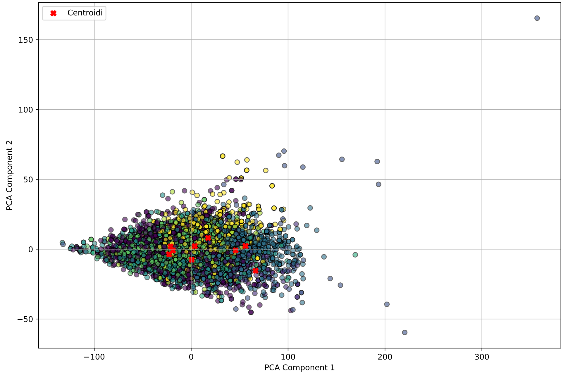
Gaussian_mixtures Clusters in PCA Projection (white wines)
